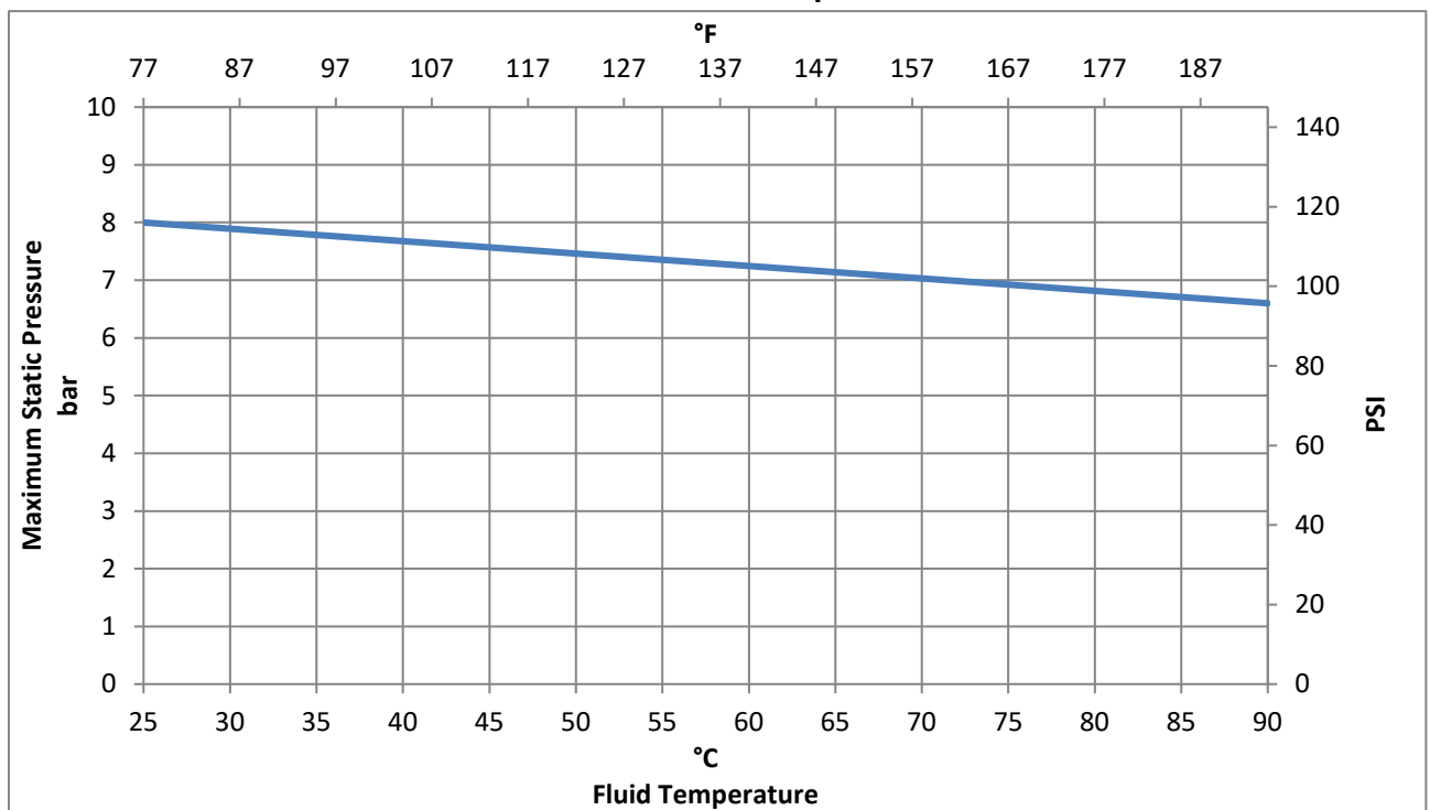
Figure 6 – Maximum Static Pressure Allowed vs. Fluid Temperature
