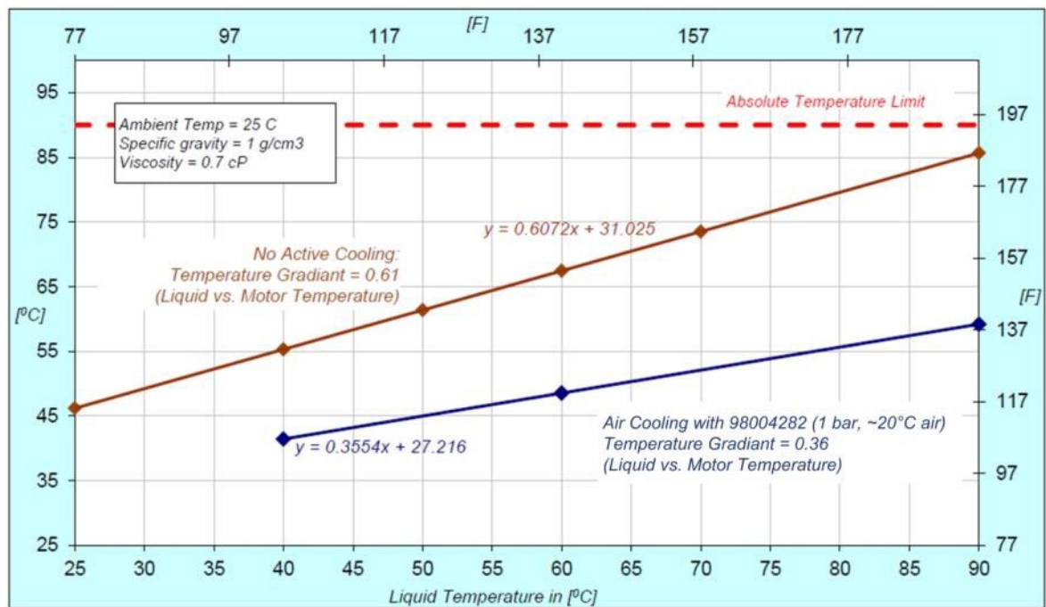
Figure 19 – Fluid Temperature Influence on Motor Temperature (Measurement at 7000 RPM, 23 LPM but gradients are representative for other operational points)
