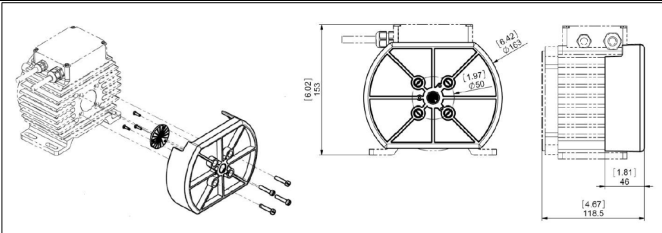
Figure 11 – Motor dimensions with attached air-cooling module.
