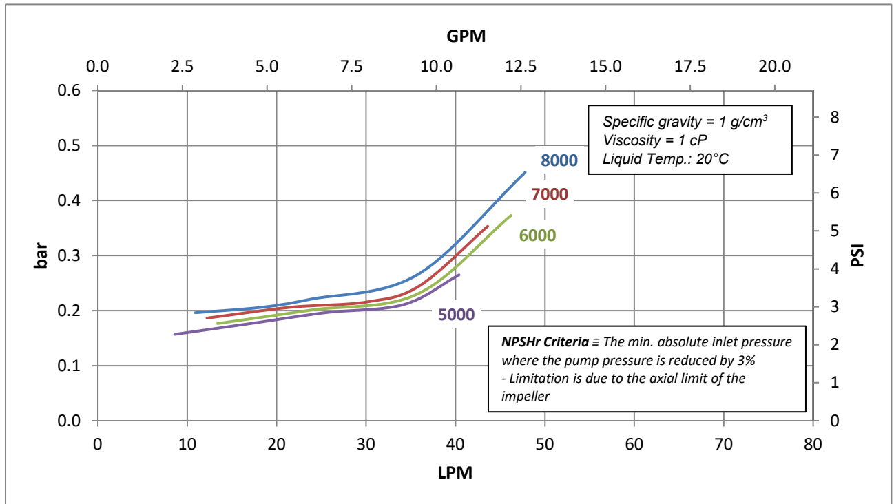
Figure 5 – NPSHr Curves
