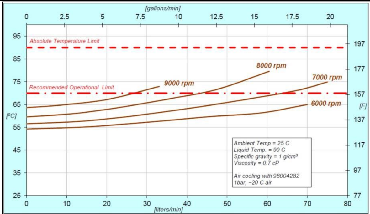
Figure 18 – Temperature Curves of Motor with Air Cooling Module (98004282)
