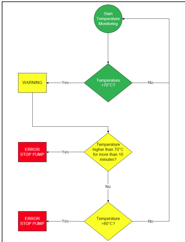
Figure 14 – Controller Temperature Monitoring
