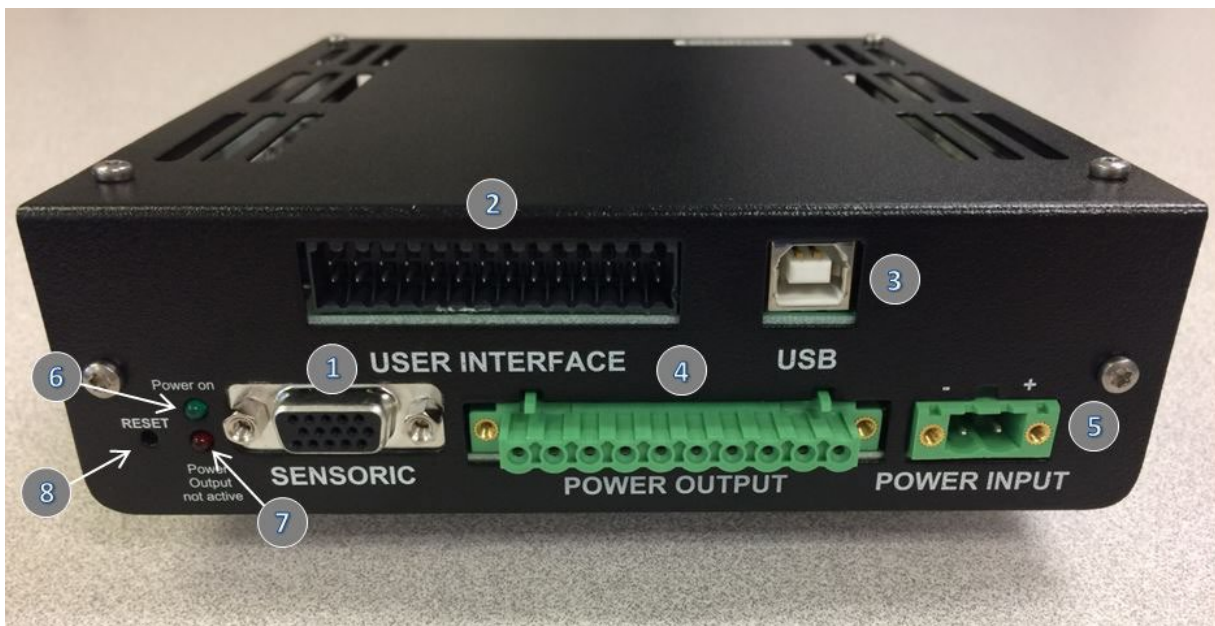
Figure 22 – Overview of the Standalone Controller Interface
