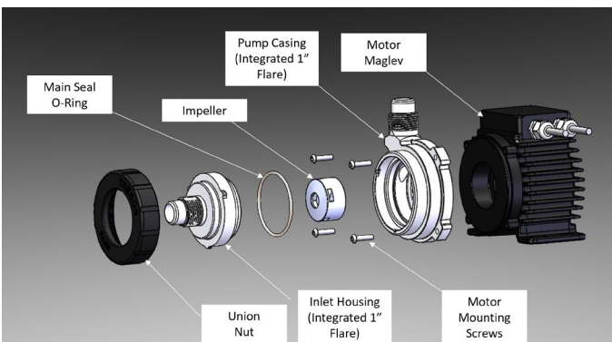
Figure 29a – Labeled Exploded View of Rev6A2 & Rev6A3 Configurations
