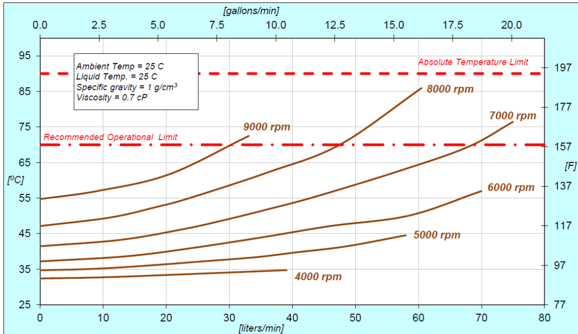
Figure 16 - Temperature Curves of the Motor for 25°C Fluid Temperature (Temperature is measured inside of the motor, contact temperature of surface is below this temperature)
