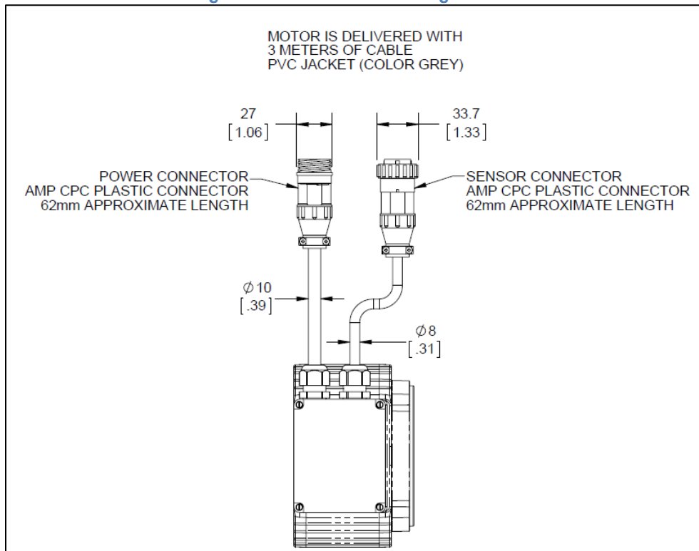
Figure 9 – Cable and Connector Specifications
