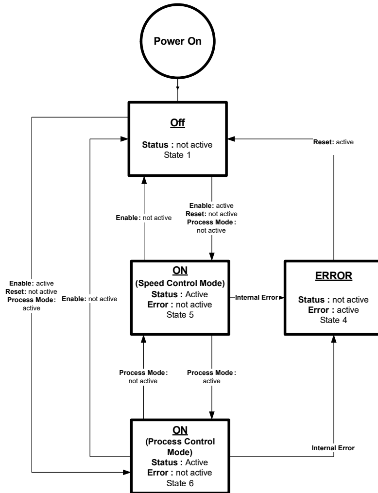
Figure 28 – PLC Interface State Diagram
