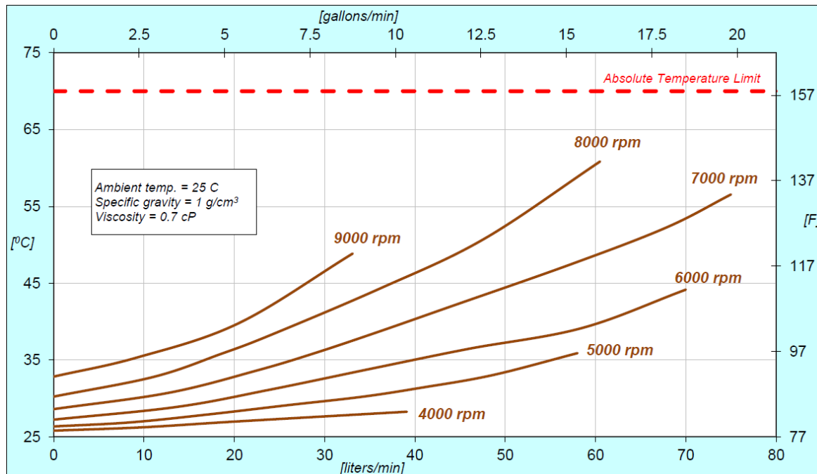
Figure 20 - Temperature Curves of Controller vs. Flow and Speed
