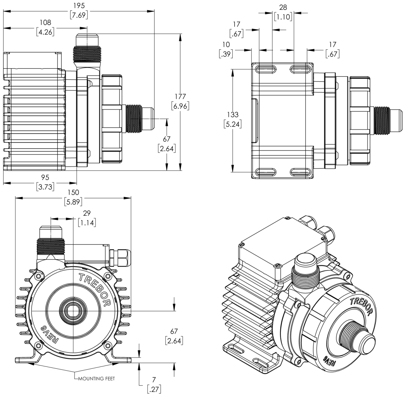
Figure 7a – Basic Pump Dimensions (Rev6A2 & Rev6A3)
