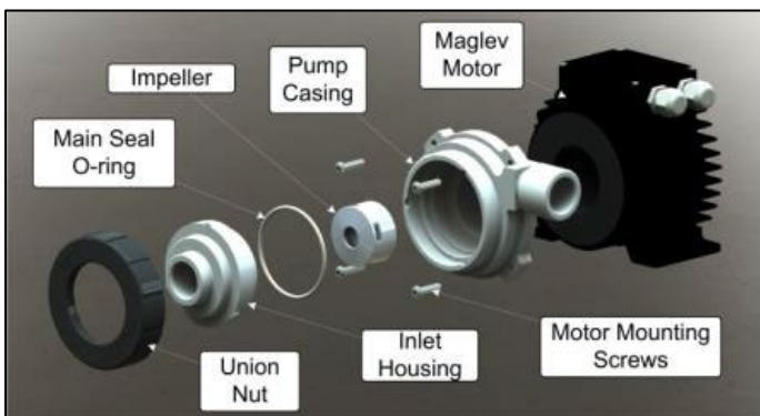
Figure 29 – Labeled Exploded View of Pump
