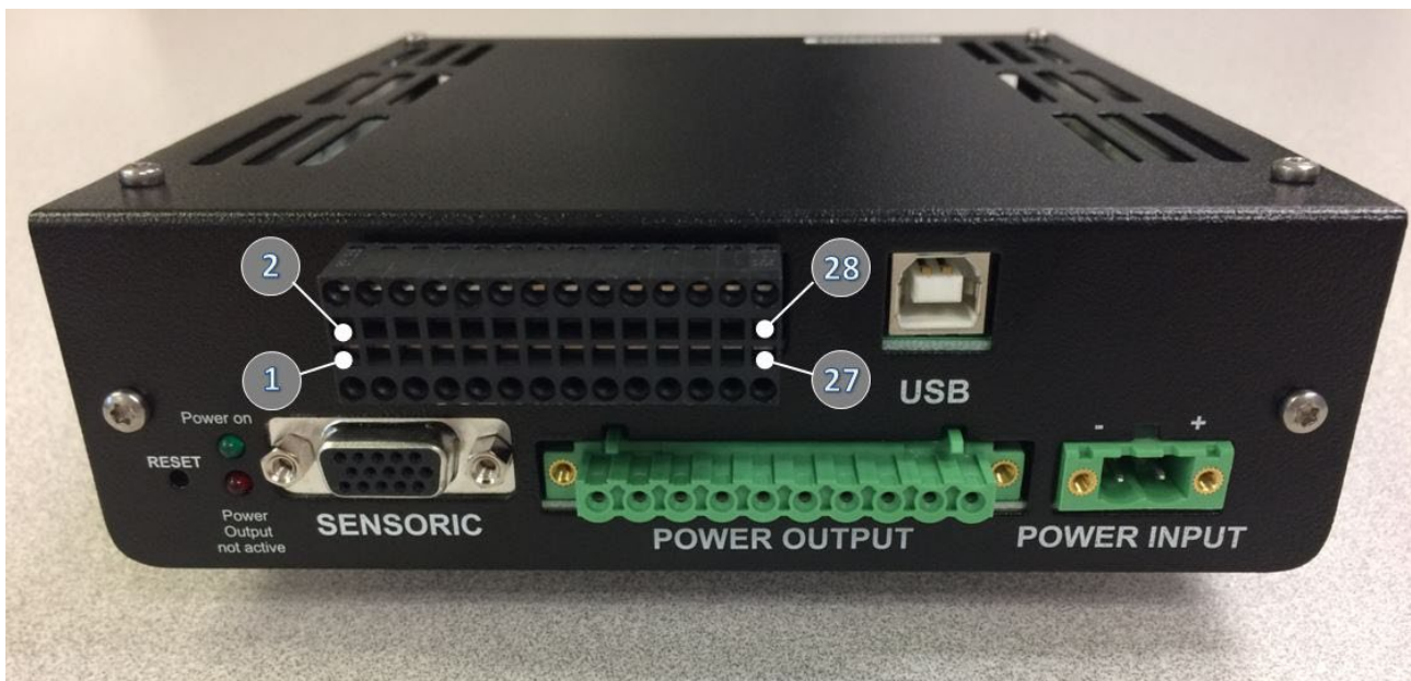
Figure 26 – Mounted PLC connector and Pin Numbering
