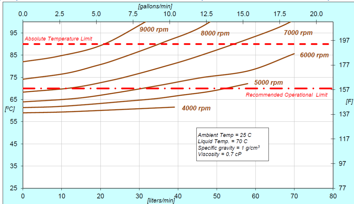
Figure 17 - Temperature curves of the Motor for 70°C Fluid Temperature (Temperature is measured inside of the motor, contact temperature is below this temperature)
