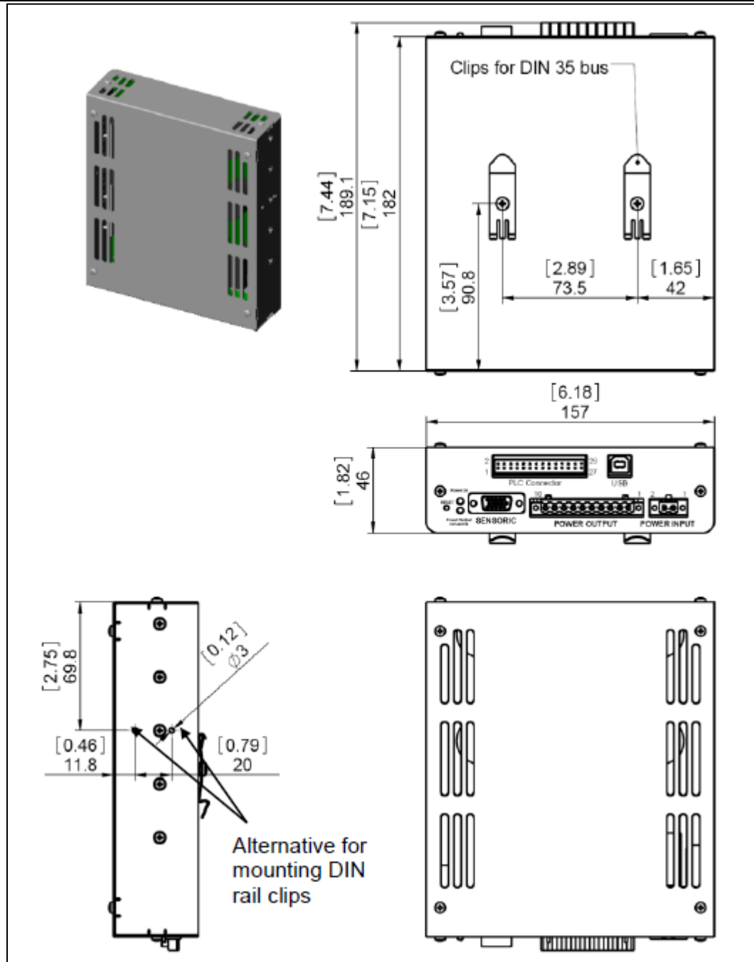
Figure 10 – Controller Basic Dimensions
