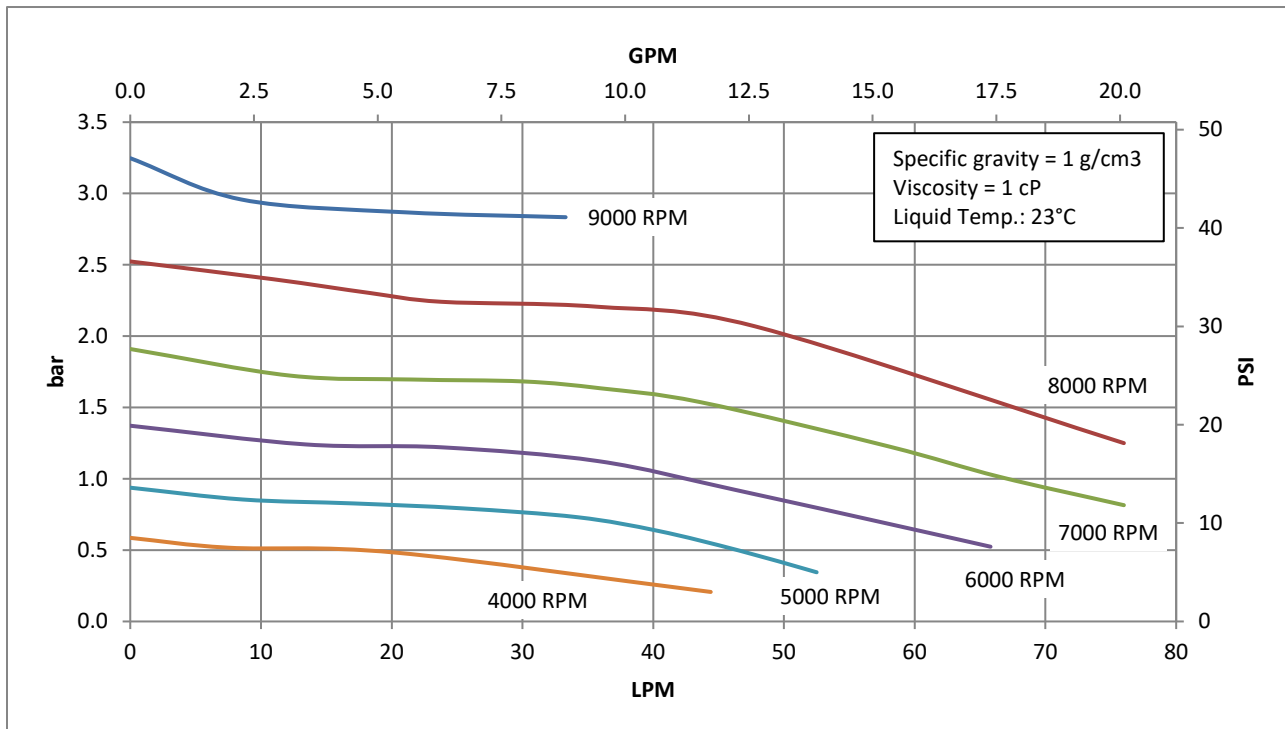
Figure 4 – Rev6 Flow vs Diff Pressure Curves
