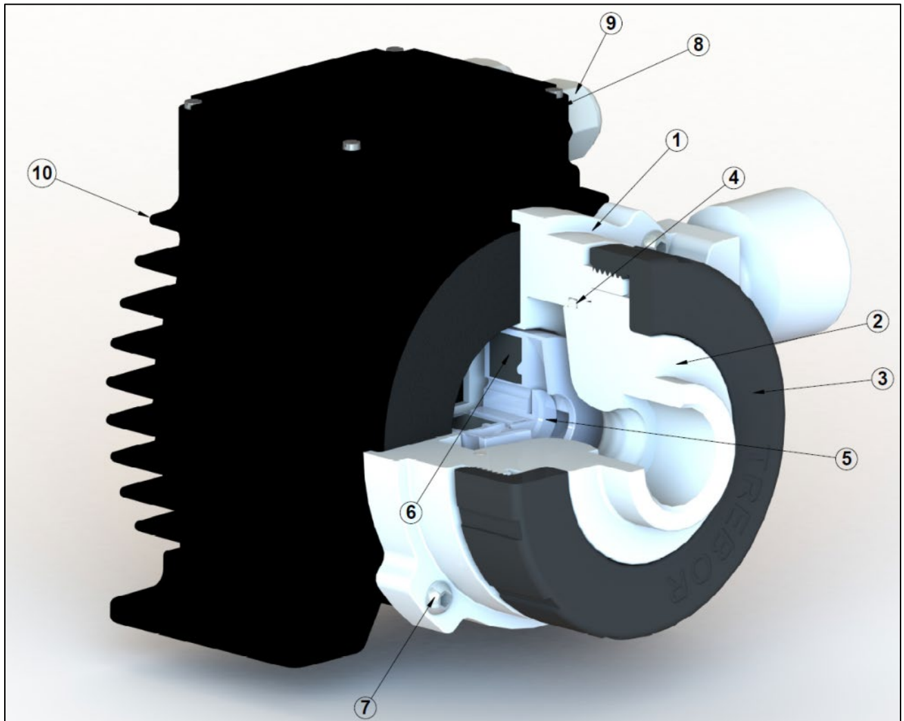
Figure 12 – Sealing and Material Concept
