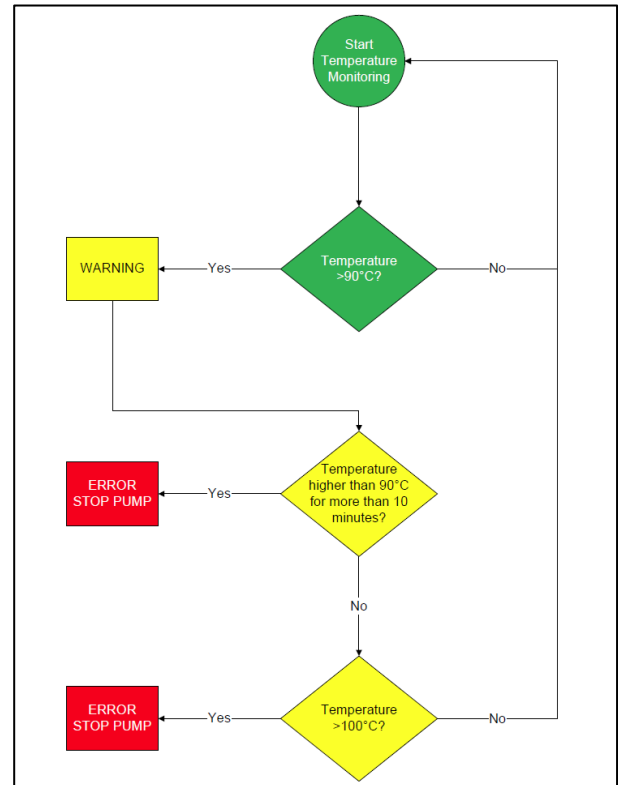
Figure 15 – Motor Temperature Monitoring
