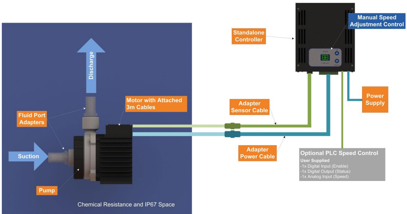
Figure 2 – Standard System Configuration for Standalone Control (Rev6A0 or Rev6A2)
