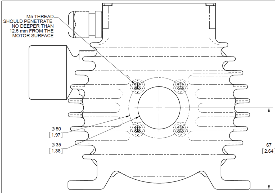
Figure 8 – Alternative Mounting Position
