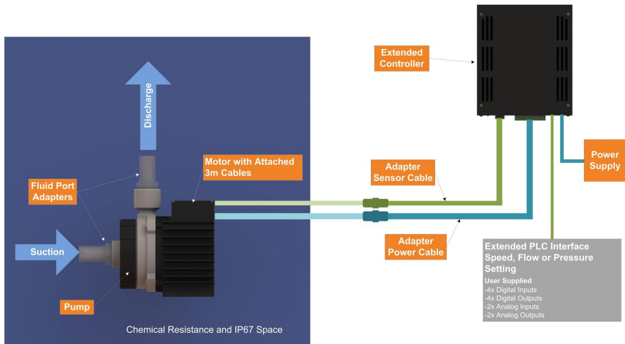
Figure 3 – Extended System Configuration for Extended Control (Rev6A1 or Rev6A3)
