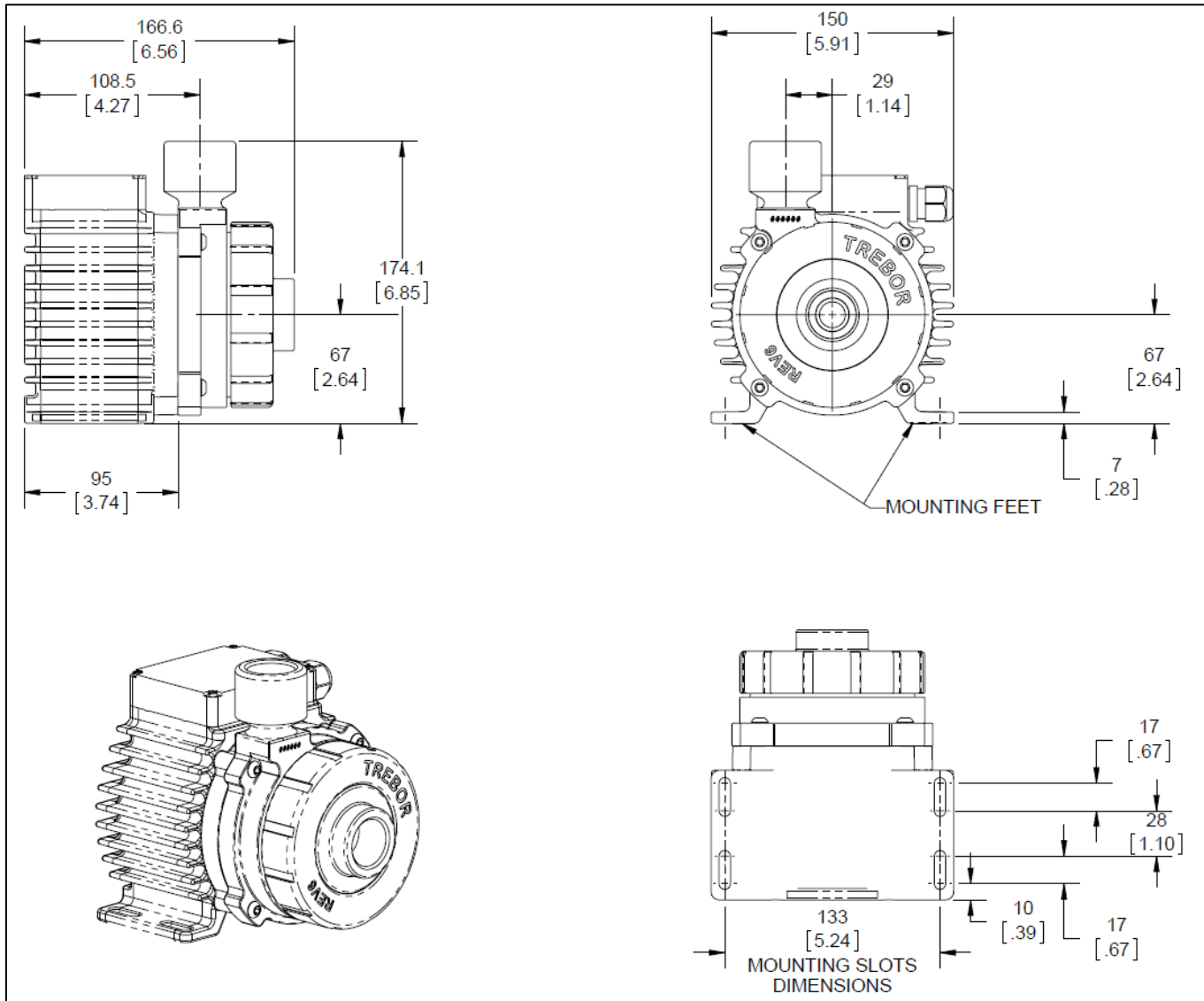
Figure 7 – Basic Pump Dimensions
